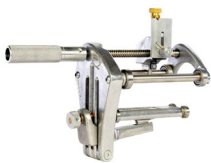
Uniprep 400 Rotary Scraper
